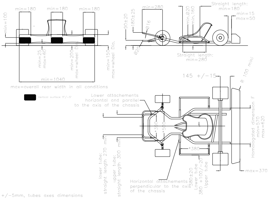
DRAWING 18a MINIKART BUMPERS & REAR PROTECTION
